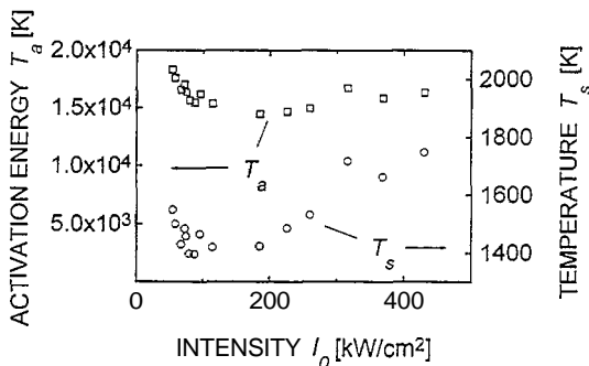
Fig. 3. The temperature of stationary ablation T_s (circles) and the activation energies T_a (squares) calculated from t_v and v depicted in Fig. 3.
