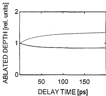
Fig. 7. The calculated dependence of ablated thickness on the delay time between the pulses in a two-pulse experiment. Calculations are done for the thermal model. Solid line: bleaching ( s=0 ); dashed line: darkening ( s=3 ). Ablated depth is normalized to its value for zero delay time.
